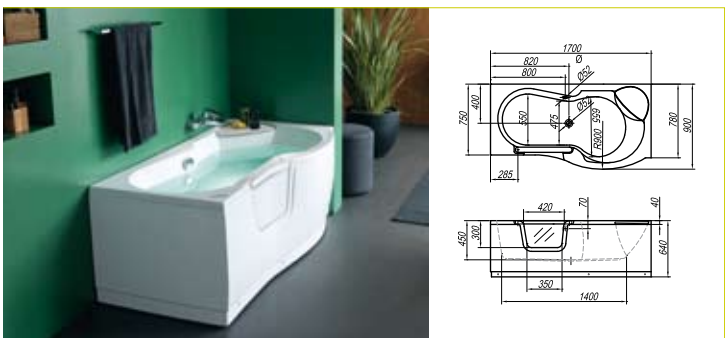
Green line D x Š x G x (VM) vol 170 x 90 x 45(64) 250 l
