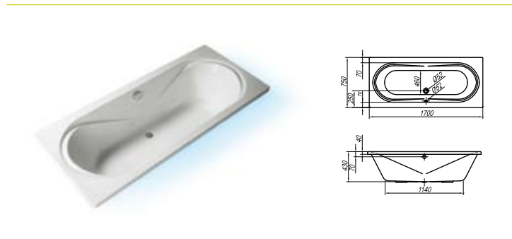
Green line D x Š x G x (VM) vol 170 x 75 x 43 (61) 215 l
